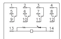
AC wiring diagram
