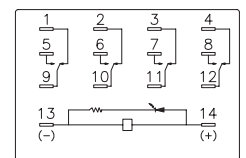
DC wiring diagram
