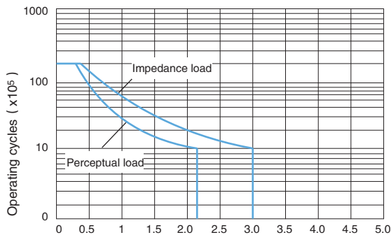
Electrical Life Curve
