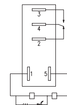
AC wiring diagram
