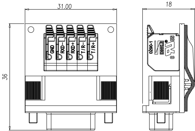
RS485 Adapter
