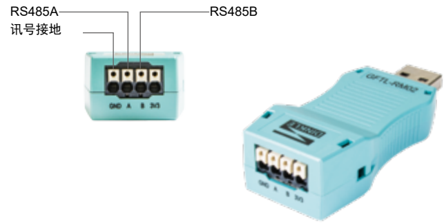
USB / RS485
