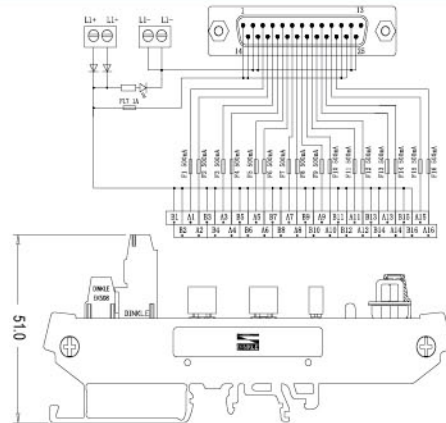
D_Sub Connector Pin Assignment
