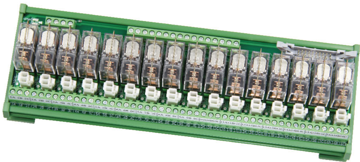
跳接线1x16pcs
