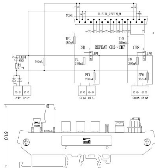
D_Sub Connector Pin Assignment
