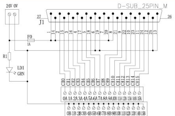
Pin Assignment
