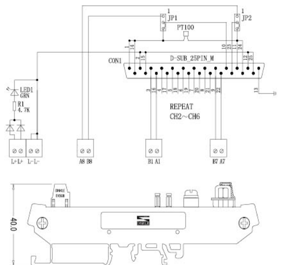
D_Sub Connector Pin Assignment
