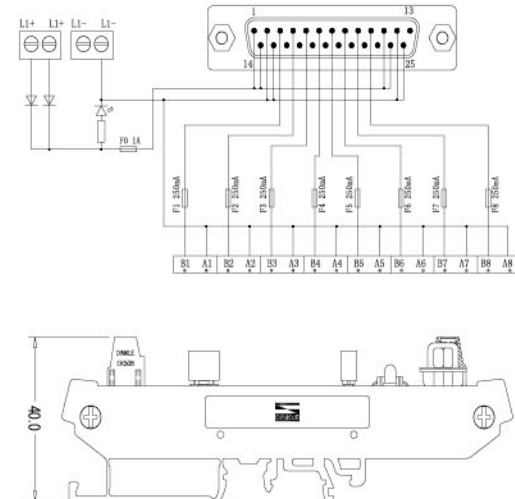
D_Sub Connector Pin Assignment
