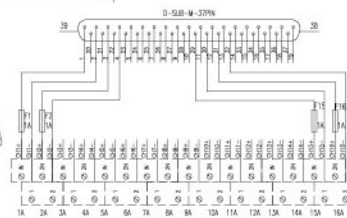
D_Sub Connector Pin Assignment
