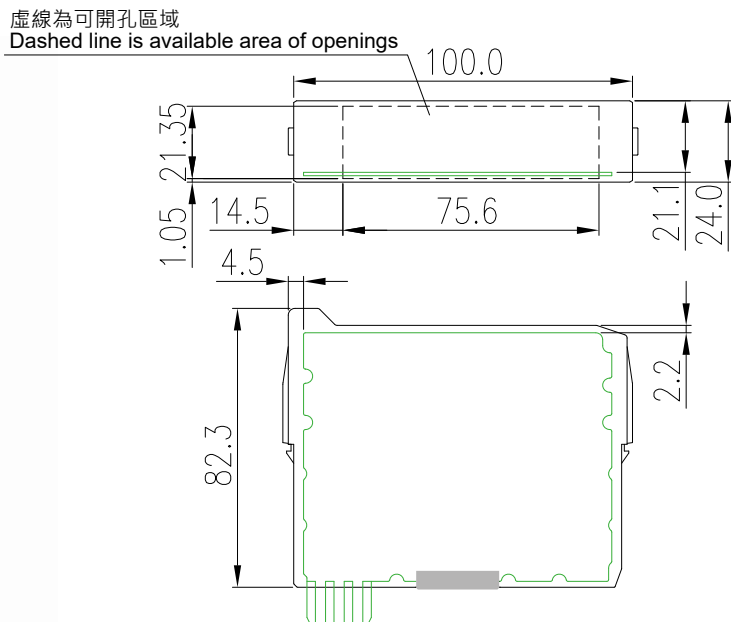
尺寸 / Dimensions: 100 x 82.3 x 24 mm (L x H x W) 材質 / Material : PC
