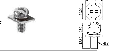
Screw
