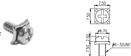
Screw
