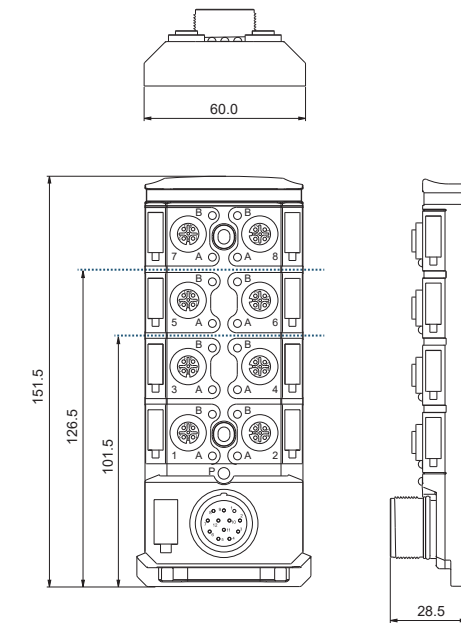
Pluggable M23 Connector
