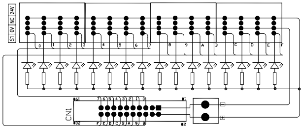
0241-C120K Wiring Diagram
