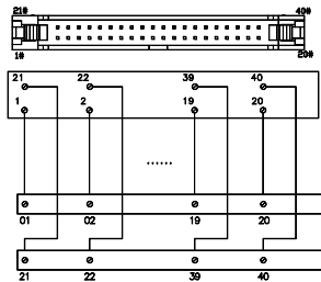
0241-C1XXSWiring Diagram
