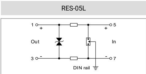
Two-wire system
