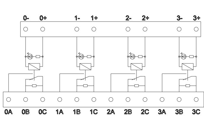
Wiring Diagram
