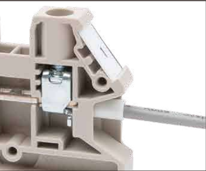
Screw connection
